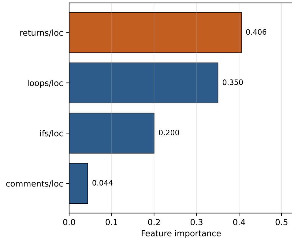
Config C: per-LOC normalized
