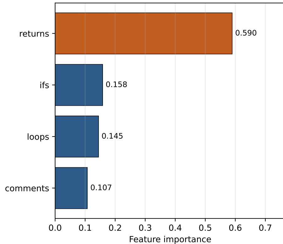
Config B: without LOC
