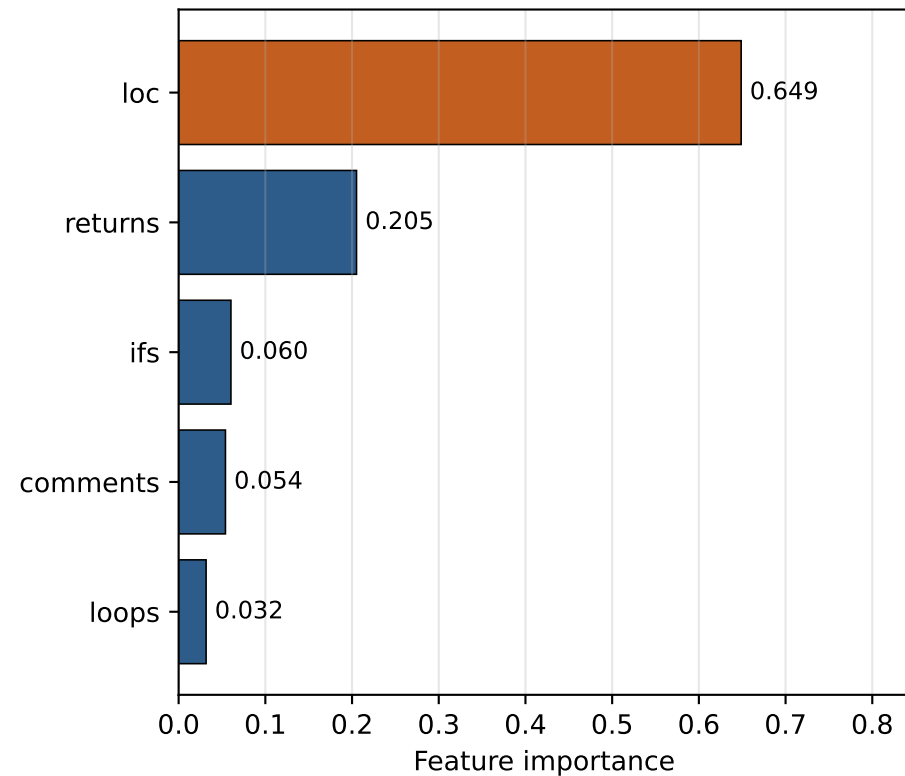
Config A: all 5 features
